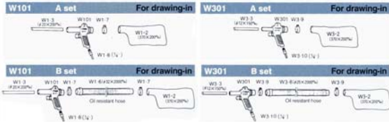
W101 Nozzle ID=Ø22mm
